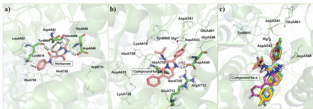
Figure 4. (a) Merbarone, (b) compound 6a , and (c) alignment of compounds 6a–e in the merbarone-binding pocket of hTopoII \alpha . Red dashed lines represent the \pi - \pi , cation- \pi , and \text{NH}-\pi interactions. Black dashed lines are hydrogen bonding interactions. \text{Mg}^{2+} is shown as a nonbonded sphere (magenta). Residues that are involved in hydrogen bonding are shown in stick presentation. For clarity, only polar hydrogens are displayed.
